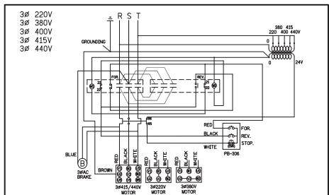
Switch with an emergency stop button
